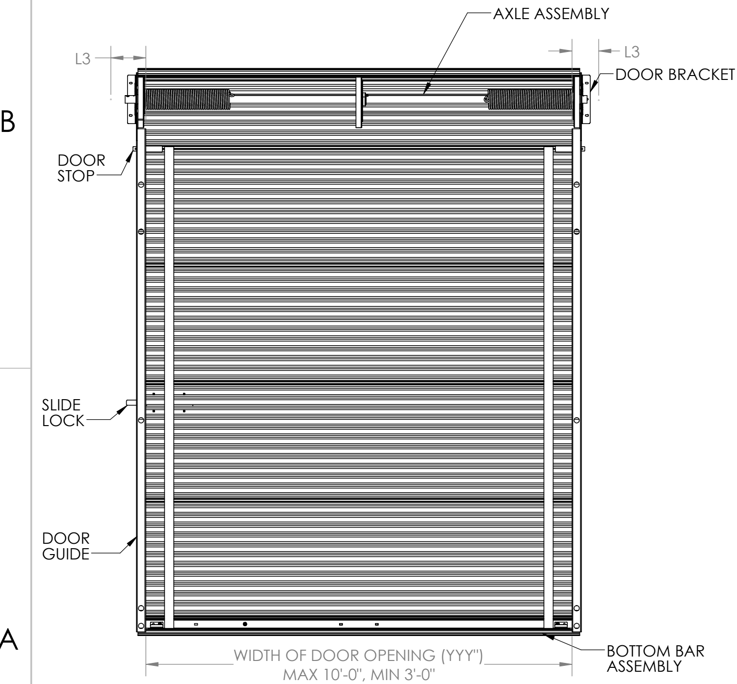
INSIDE ELEVATION
