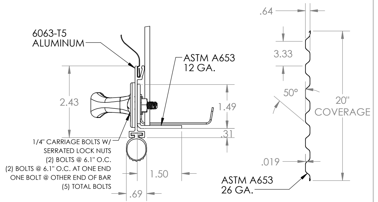
BOTTOM BAR ASSEMBLY DETAIL
