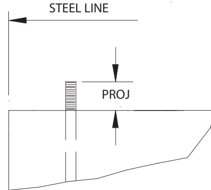
ANCHOR BOLT PROJECTION
