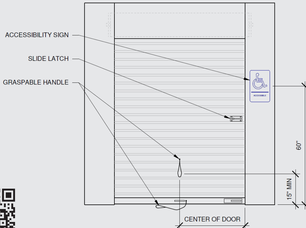
CLOSED ROLL-UP DOOR FRONT ELEVATION
